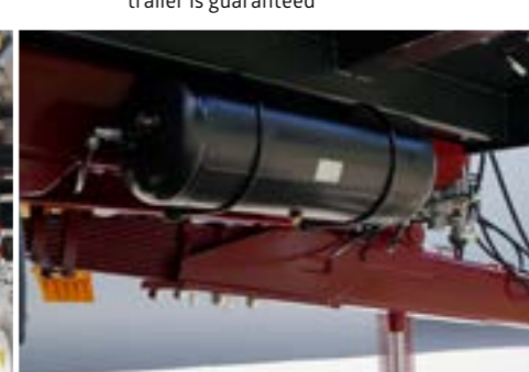
Sprung drawbar increases driving comfort
